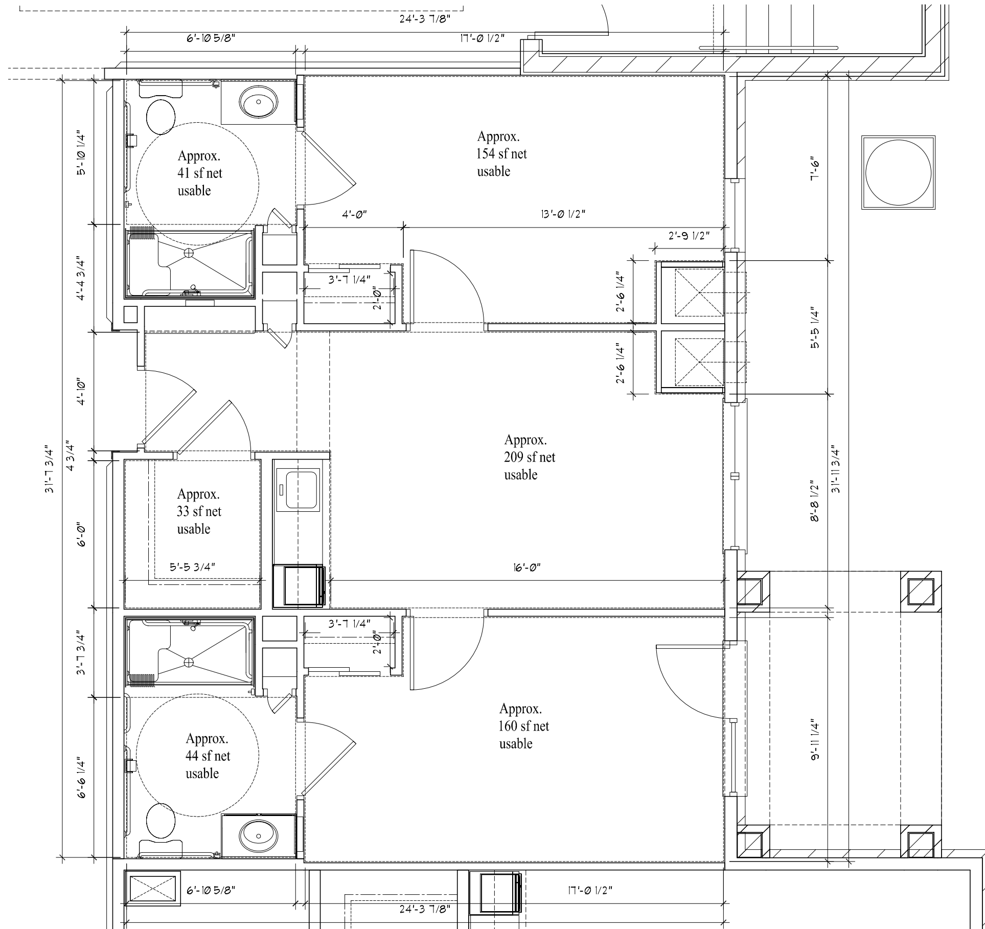
Assisted Living Unit Type C 1/4" = 1'-0" 791 sf gross
